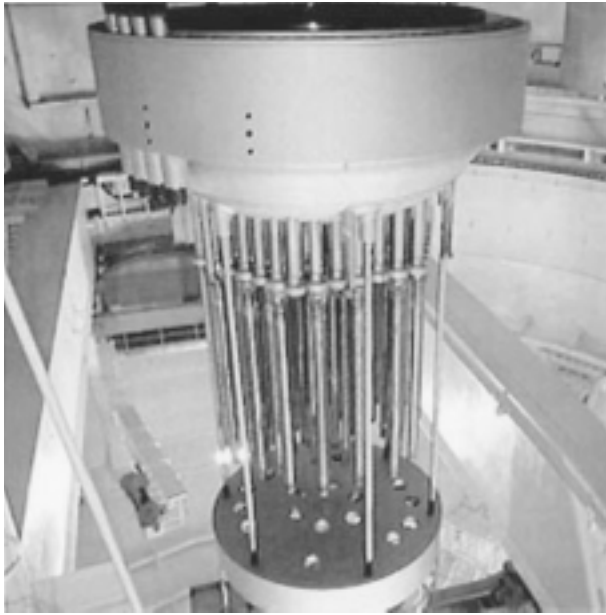
(a) VVER fuel rod assembly
