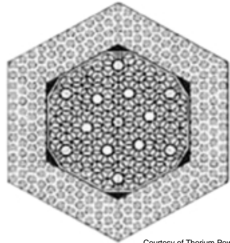
(b) Radkowsky design for the thorium seed/blanket assembly. The seed fuel is the inner part of the fuel rod (three-sectioned), and the blanket fuel is the outer part. The thorium fuel assembly is designed to replace the current fuel assembly, without requiring a major design overhaul.
